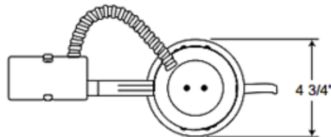
4 3/8" CEILING CUTOUT
