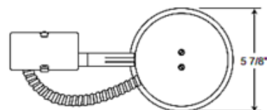
5 1/2" CEILING CUTOUT
