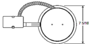
6 3/4" CEILING CUTOUT
