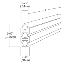
Monorail 2 Circuit Overall Dimensions
