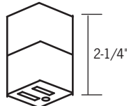
LA-1B 15/16" Grid Deep Tile T-Bar Clip. Fits into channel in back of track. May be spaced to 4'. Finish: -S
