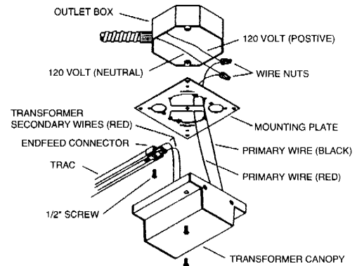
TL546, TL566U CANOPY TRANSFORMER
