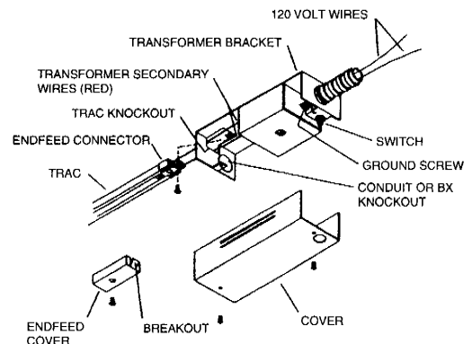
TL547, TL567U SURFACE TRANSFORMER
