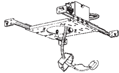
FRAME-IN KIT
