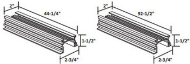
RTH-4 Housing for 4' Track Sections Use with LT-4 or LT-24.
