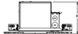
4 1/2" CEILING CUTOUT
