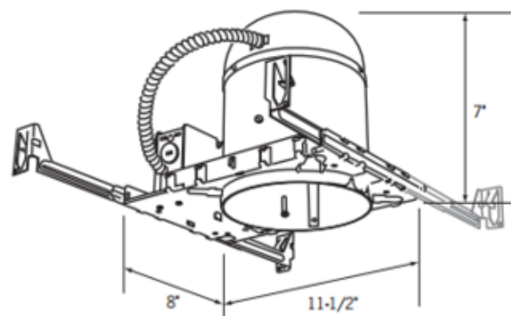
Ceiling Opening: 5-3/4"
