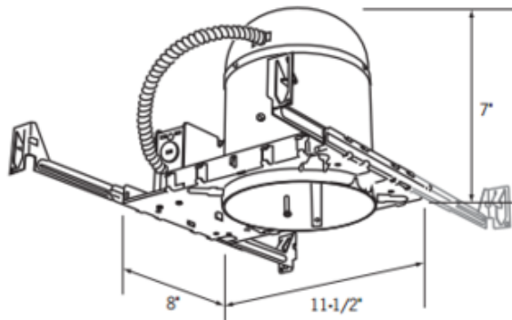
Ceiling Opening: 5-3/4"
