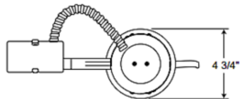
4 3/8" CEILING CUTOUT
