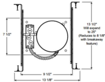
6 7/8" CEILING CUTOUT
