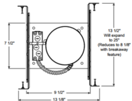
6 7/8" CEILING CUTOUT
