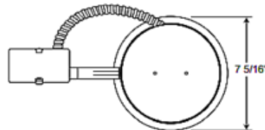
6 3/4" CEILING CUTOUT
