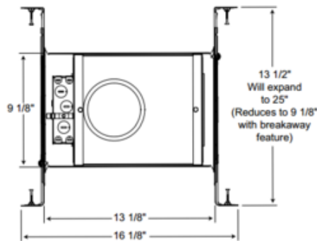
4 1/2" CEILING CUTOUT
