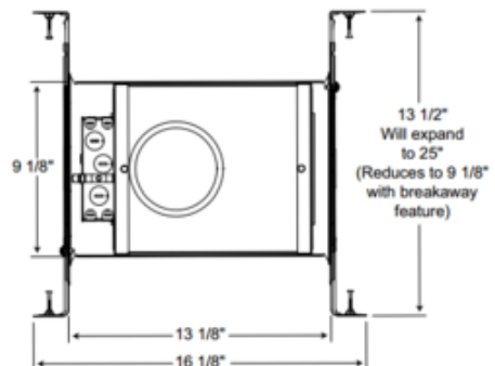
4 1/2" CEILING CUTOUT
