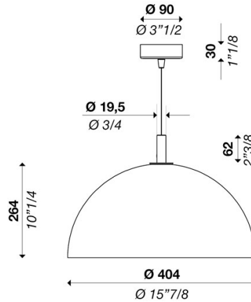
Technical drawing Size ref. image mm - inch
