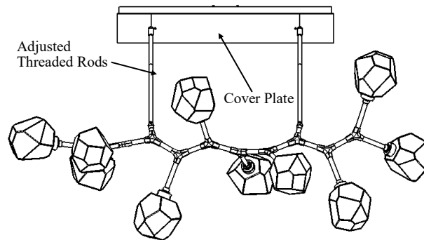
Fixture before End glass pieces are attached. Example (PLB0061-50)
