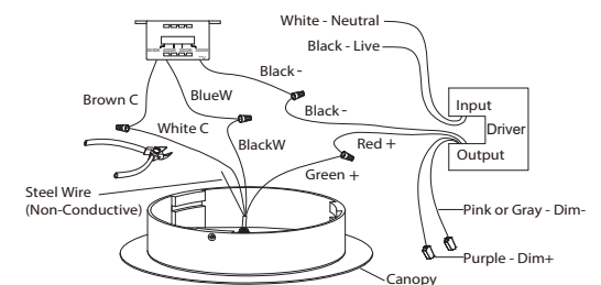
Fig.4 Driver Wires
