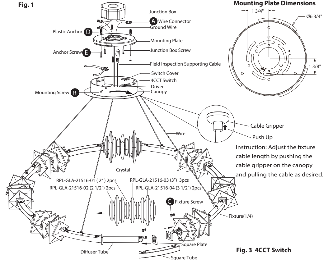
Mounting Plate Dimensions
