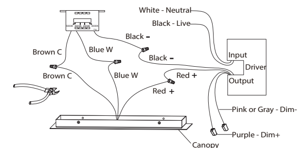
Fig.4 Driver Wires
