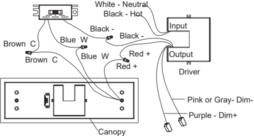
Fig. 3 Driver Wires
