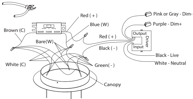
Fig. 4 Wire Diagram
