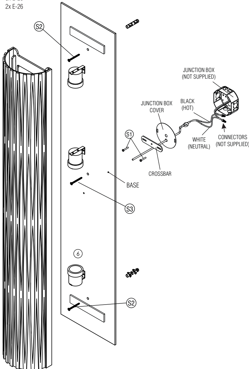
PROVIDED SCREWS
