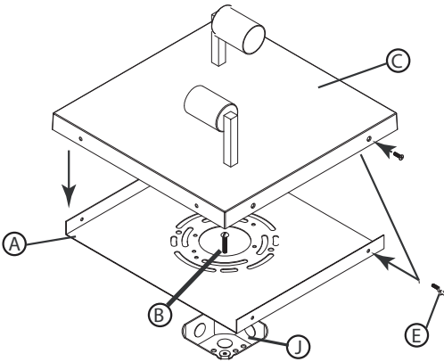
DRAWING 2 - INSTALLATION
