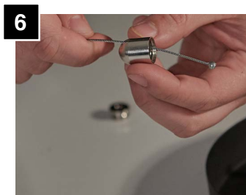
Completely feed aircraft cable through coupler, until stop is reached.
