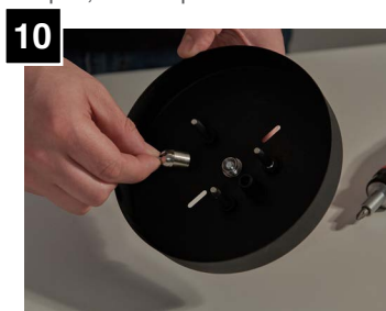
Twist and tighten coupler with aircraft cable to coupler end cap.
