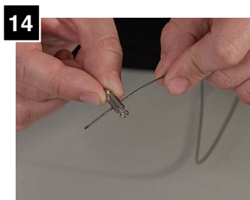
Pass aircraft cable through one hole of strain relief.
