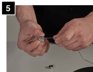
Twist off end cap from cable coupler and feed aircraft cable.
