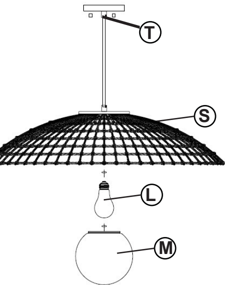
DRAWING 2- ASSEMBLY
