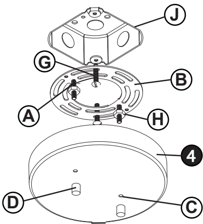
DRAWING 1- MOUNTING
