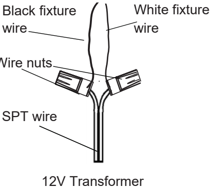
DRAWING 2- Multiple fixture wiring
