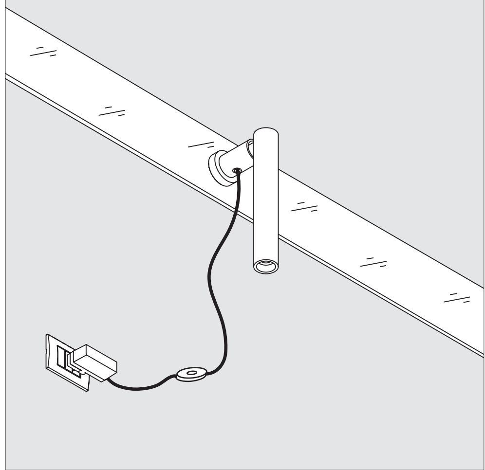
Example of installation with power kit with plug
