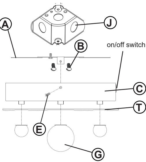
DRAWING 1 - MOUNTING
