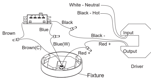
Fig.3 Wiring Diagram
