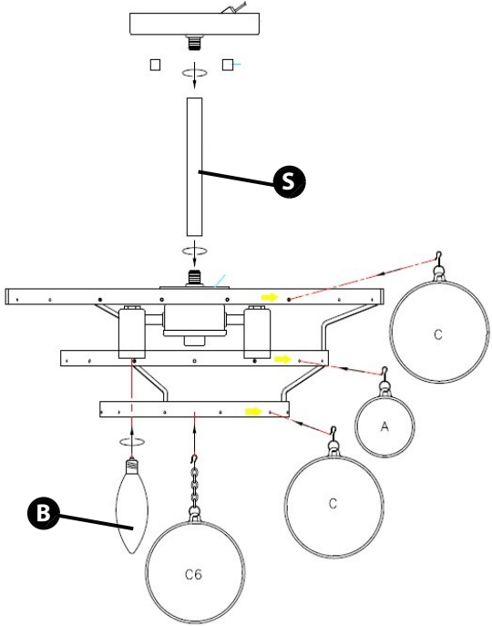
DRAWING 2 - Assembly
