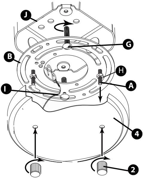
DRAWING 2 - Assembly
