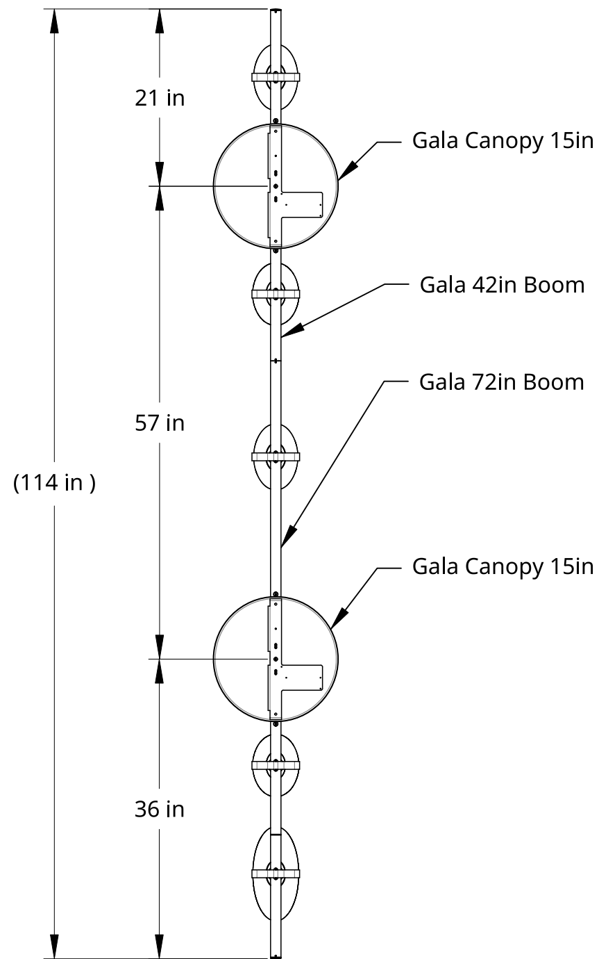
Top View: Canopy Spacing
