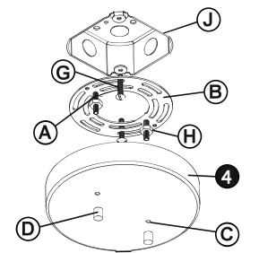
DRAWING 2- ASSEMBLY
