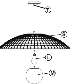
DRAWING 2- ASSEMBLY
