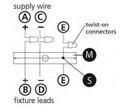
Drawing 3 – Post-Mount
