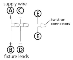
Drawing 3 – Post-Mount
