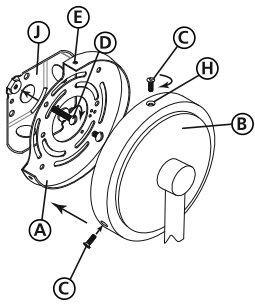
DRAWING 2 - GLASS INSTALLATION
