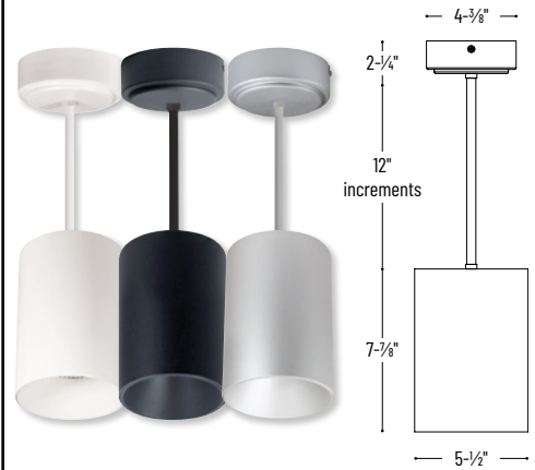
NYLM-5ST Stem Mounted
