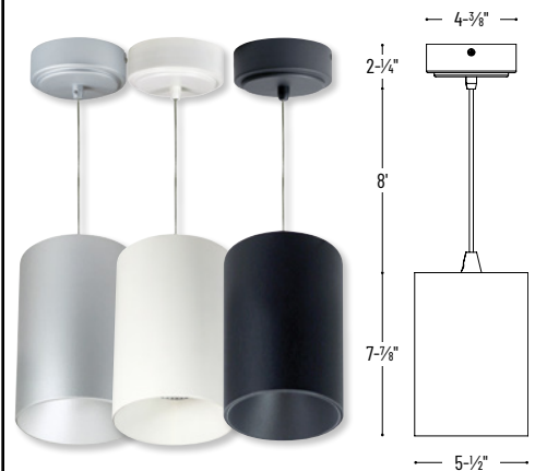
NYLM-5C Cable Mounted
