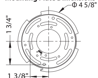
Mounting Plate Dimensions
