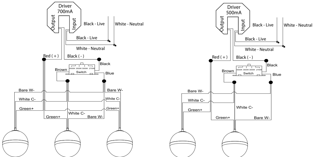
Fig. 4 Driver Wires
