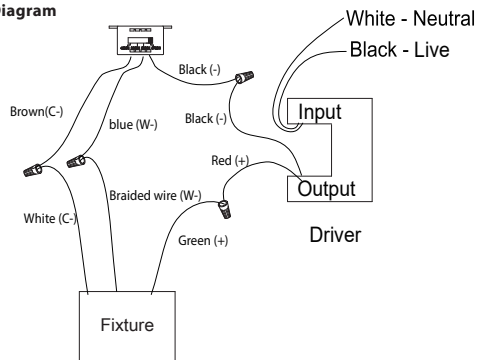
Fig. 4 Wire Diagram
