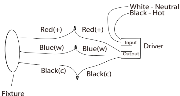
Fig.2 Driver Wires
