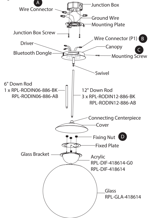
Fig. 3 Driver Wiring
