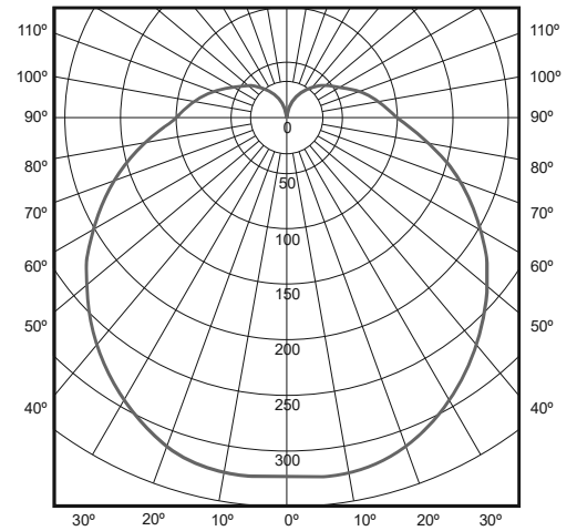
CANDLE POWER DISTRIBUTION
