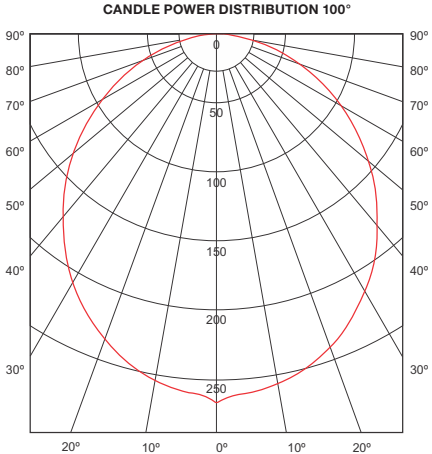
CIRRUS CEILING D1 - 100° Beam Spread
