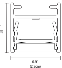
CHANNEL WITH LOUVER (ACTUAL SIZE)
