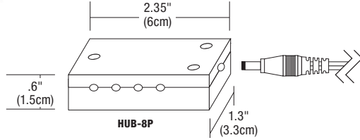
6' CORD CONNECTS TO LED POWER SOURCE
