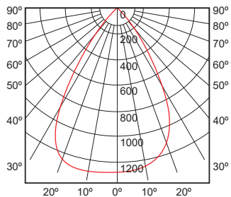
WIDE FLOOD 55°
