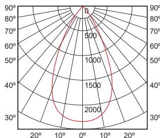
FLOOD 45°
