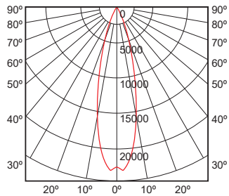
SPOT 20°
