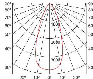
NARROW FLOOD 35°
