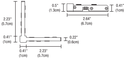
L-CONNECTOR
