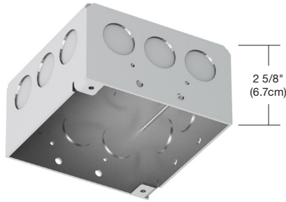
TE-60L-12 Power Supply fits in J-Box
