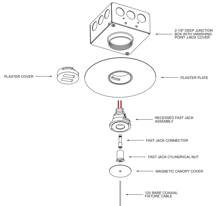
Vanishing Point 2" Flush Canopy to dry wall, plaster in and paint, with ELV power supply in J-Box
