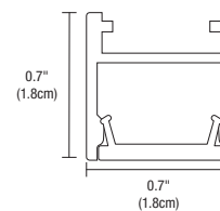
Channel Without Louver (Actual Size)
