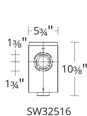
Mounting Plate
