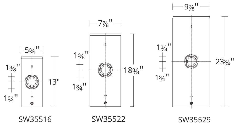
Mounting Plate
