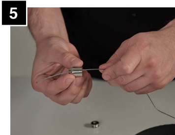
5 Twist off end cap from cable coupler and feed aircraft cable.
