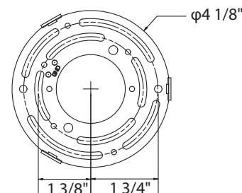
Mounting Backplate
